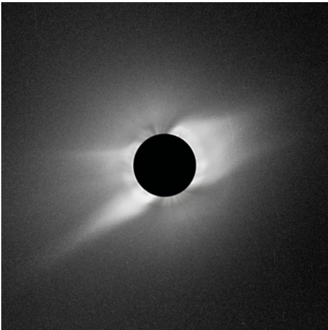
Coronal streamers during total solar eclipse G. Schneider EFLIGHT 2008 August 1
