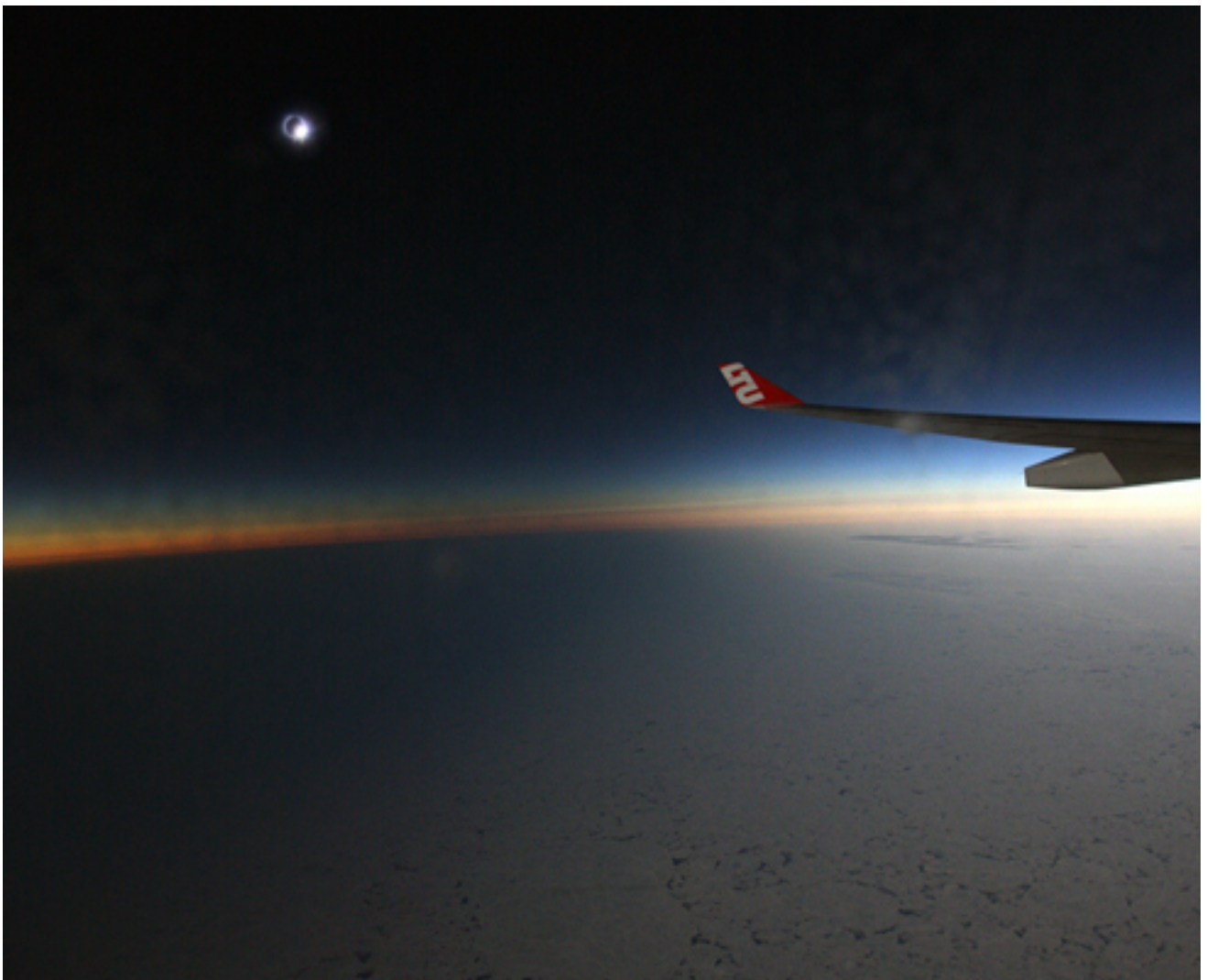
Panoramic view as moon's shadow overtakes aircraft above Arctic Ocean D. McGlaun and G. Schneider EFLIGHT 2008 August 1
